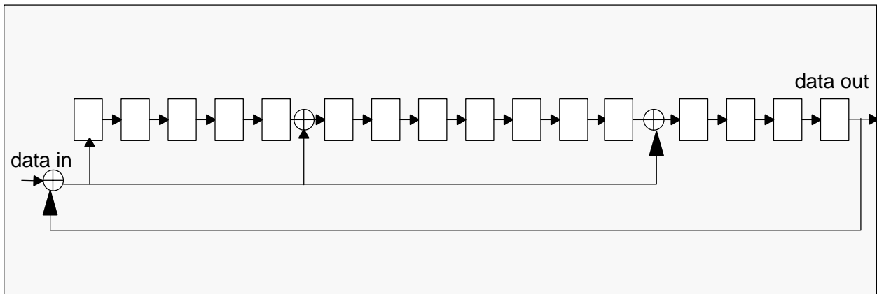
Figure 4-6: CRC16 generator/checker
