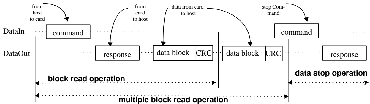
Figure 3-8: Read operation
