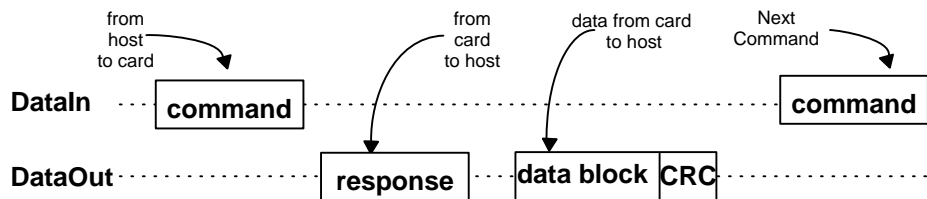
Figure 7-2: Single Block Read operation
