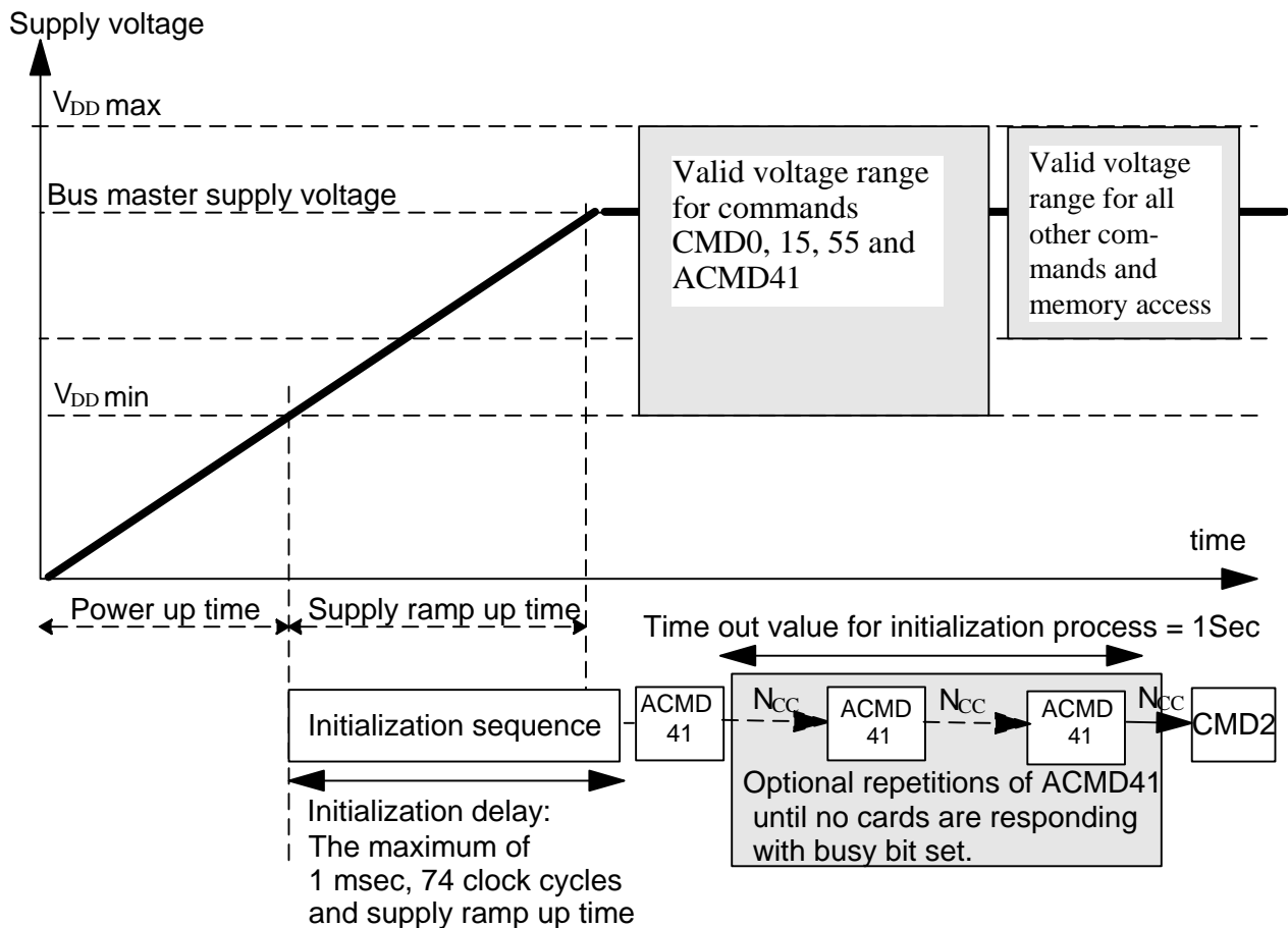
Figure 6-1 : Power-up diagram
