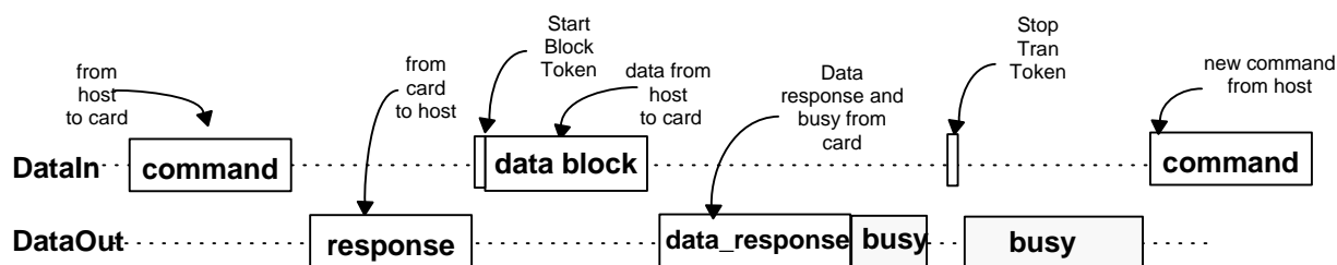
Figure 7-6: Multiple Block Write operation
