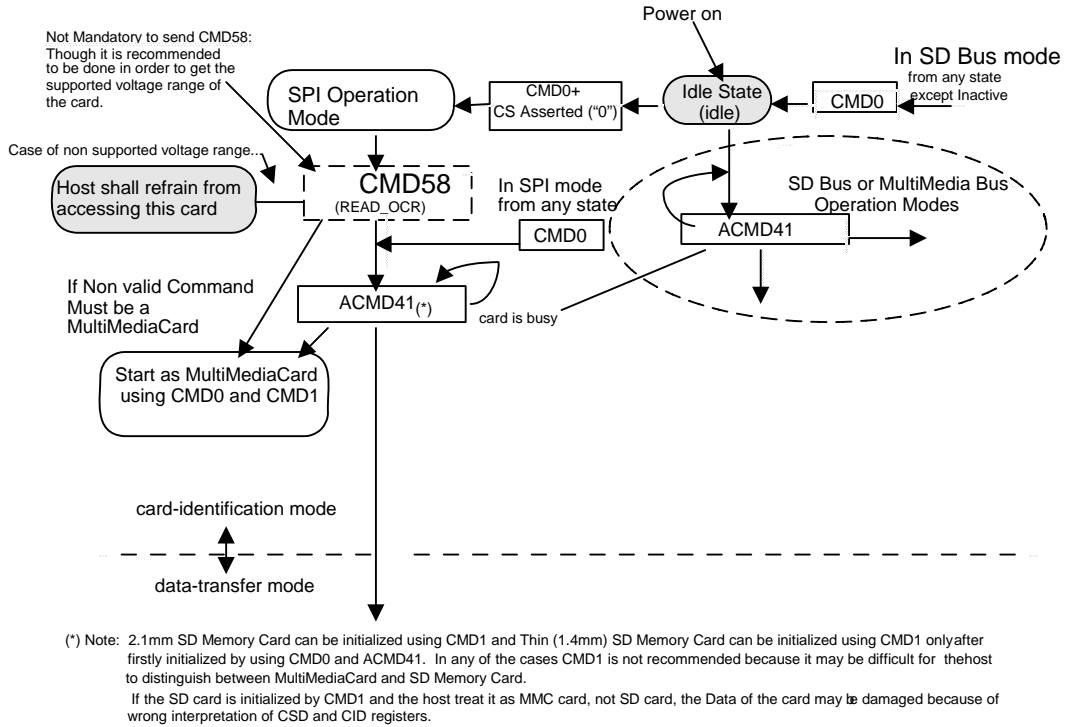
Figure 7-1: SPI Mode Initialization Flow
